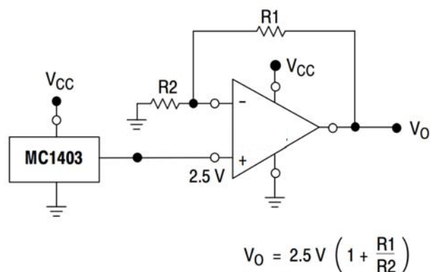
Figure 1. Voltage Reference
