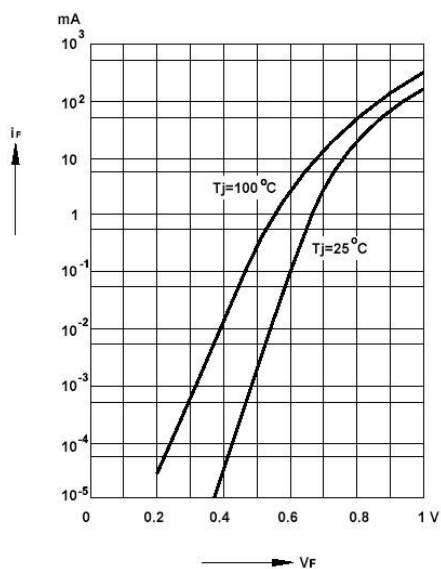
Forward characteristics
