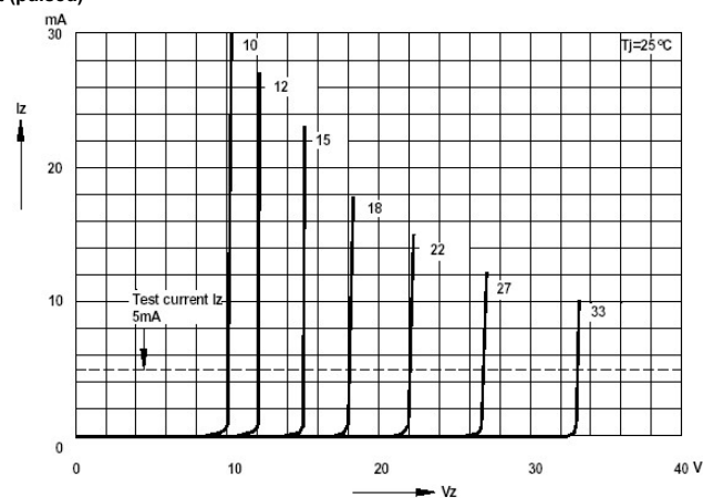
Breakdown characteristics at T_J=\text{constant} (pulsed)
