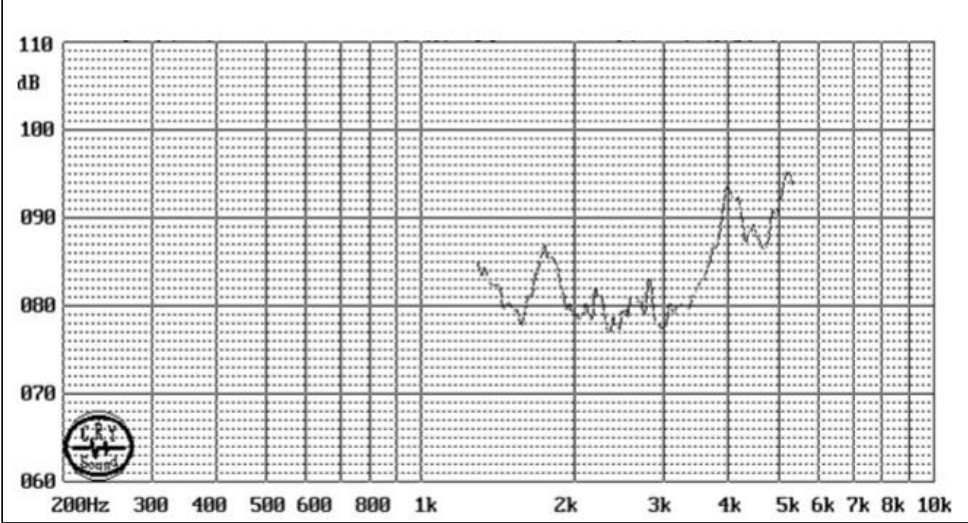
Typical Frequency Response Curve （音频曲线图）
