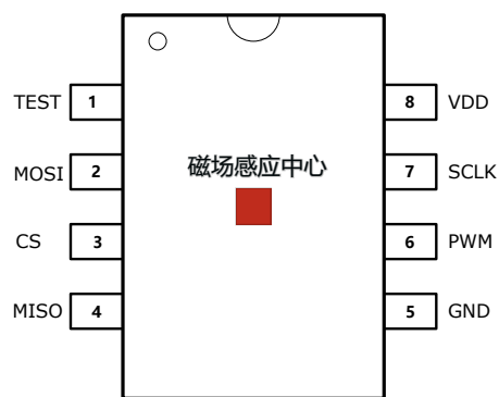
图 4: SOP-8 4.9mmx6mm
