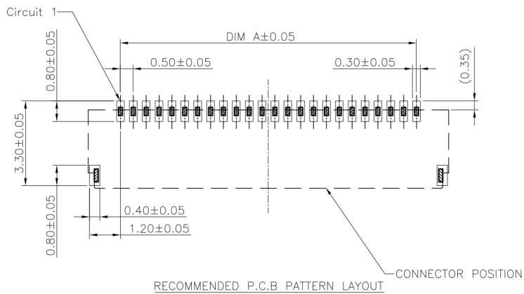
RECOMMENDED P.C.B PATTERN LAYOUT
