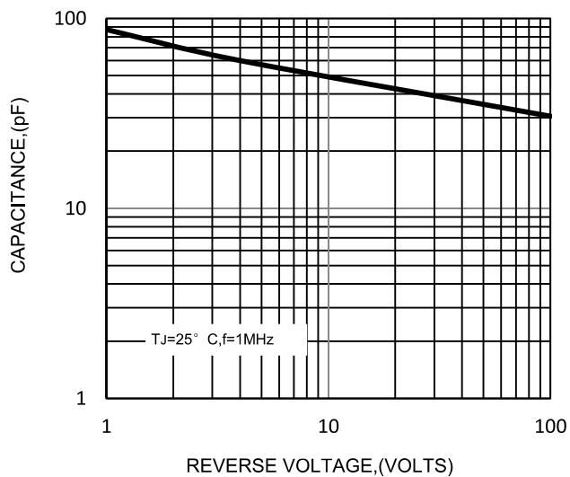
FIG.3-TYPICAL JUNCTION CAPACITANCE
