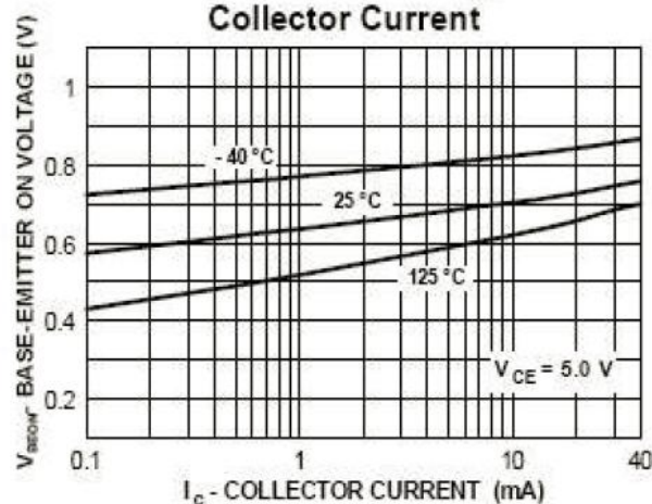
Base-Emitter ON Voltage vs Collector Current
