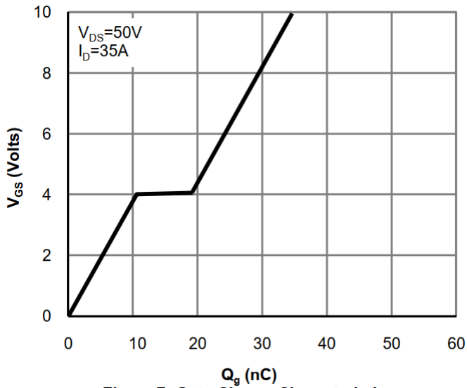
Figure 7: Gate-Charge Characteristics
