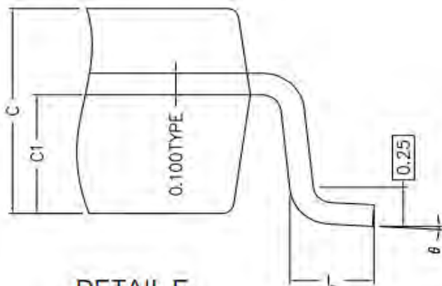
DETAIL E
