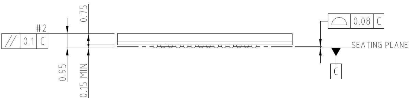
11.5 x 13.0 x 1.0mm Bottom & side View
