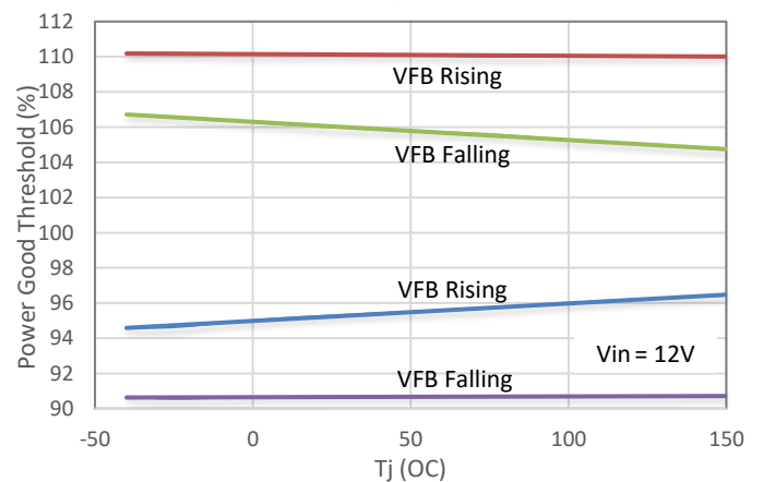
Figure 24. PG Threshold vs Junction Temperature
