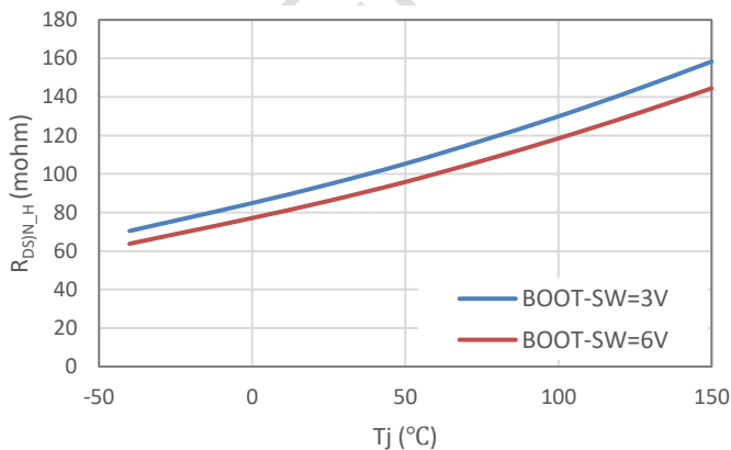
Figure 5. On Resistance vs Junction Temperature
