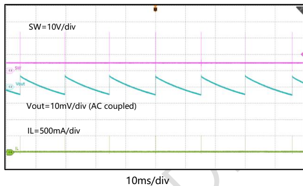
Figure 36. Output Voltage Ripple, I_{OUT}=0\text{A}
