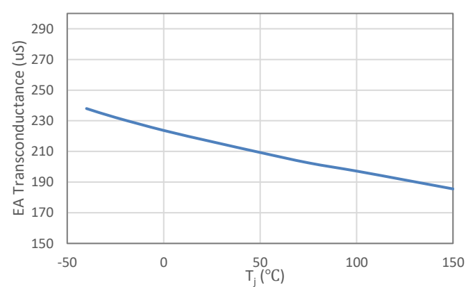
Figure 12. EA Transconductance vs Junction Temperature
