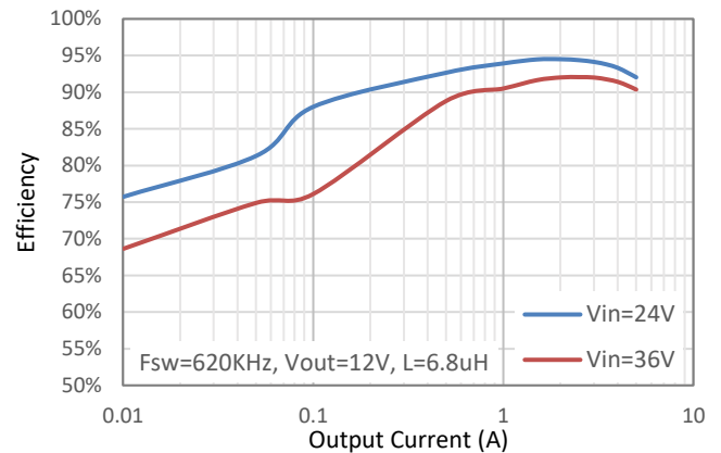
Figure 2. Power Efficiency, V_{out}=12V
