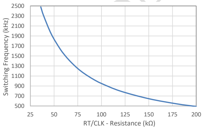
Figure 11. Switching Frequency vs RT/CLK Resistance High Frequency Range
