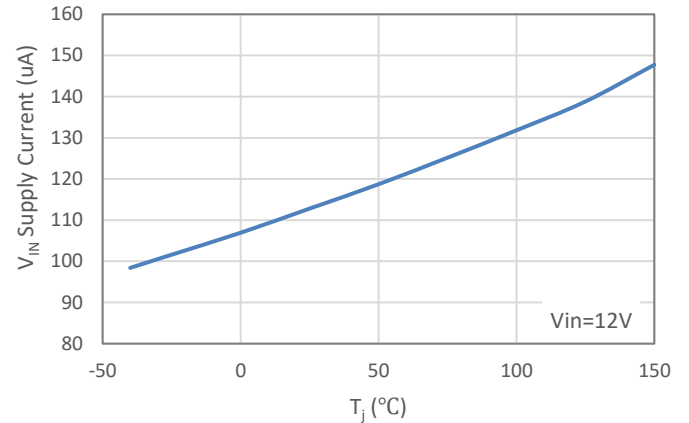
Figure 14. VIN Supply Current vs Junction Temperature
