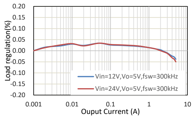
Figure 35. V_{OUT} Vs. Load Regulation
