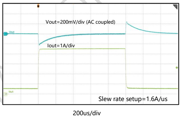
Figure 49. Transient Response 0.5A-4.5A
