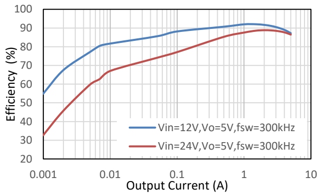
Figure 34. Power Efficiency
