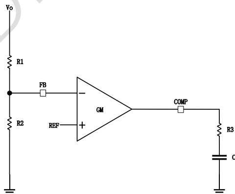
Figure 30. Loop compensation
