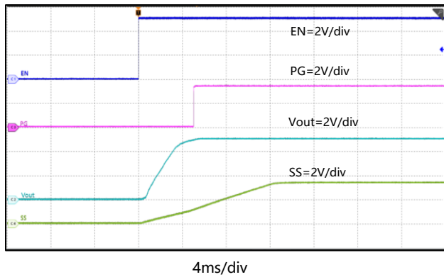
Figure 46. Start-Up with EN, I_{OUT}=5A
