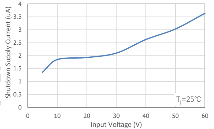
Figure 22. Shutdown Supply Current vs Input Voltage
