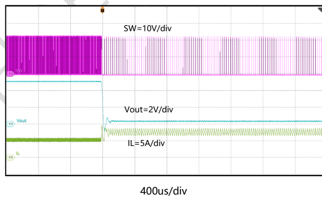
Figure 50. Normal Operation to Hard-short I_{OUT}=5A
