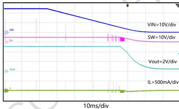
Figure 44. Shut-Down with VIN falling, I_{OUT}=0A
