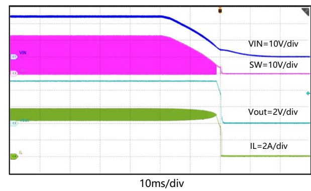
Figure 45. Shut-Down with VIN falling, I_{OUT}=5A
