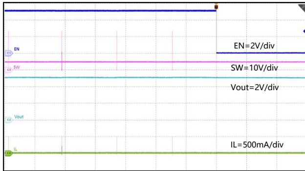
Figure 40. Shut-down with EN, I_{OUT}=0A
