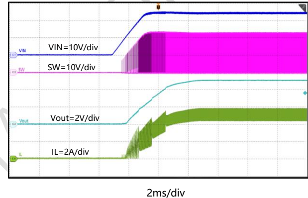
Figure 43. Start-Up with VIN Rising, I_{OUT}=5A
