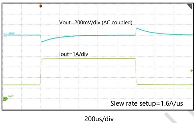
Figure 48. Transient Response 1.25A-3.75A
