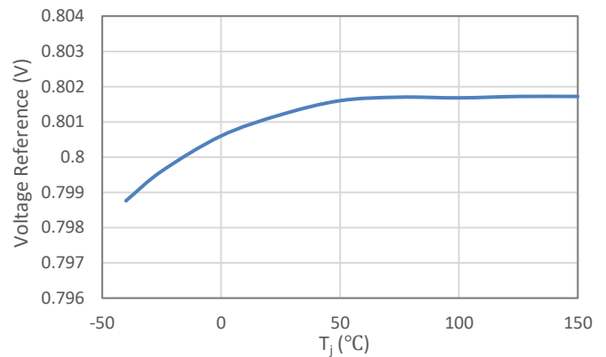
Figure 6. Voltage Reference vs Junction Temperature
