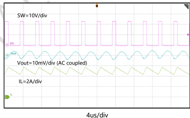
Figure 37. Output Voltage Ripple, I_{OUT}=5\text{A}
