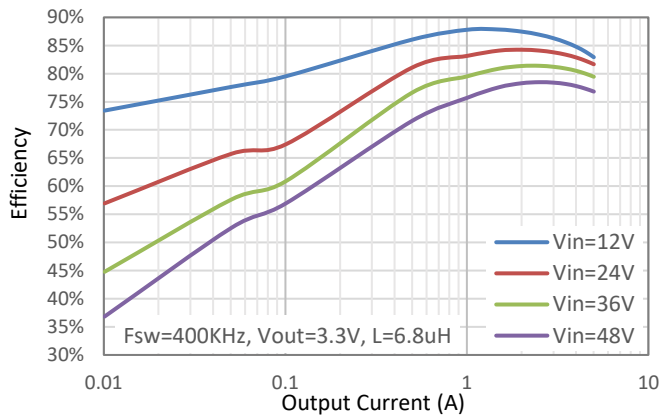
Figure 1. Power Efficiency, V_{out}=3.3V
