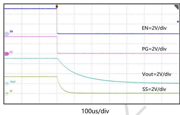
Figure 47. Start-Up with EN, I_{OUT}=5A
