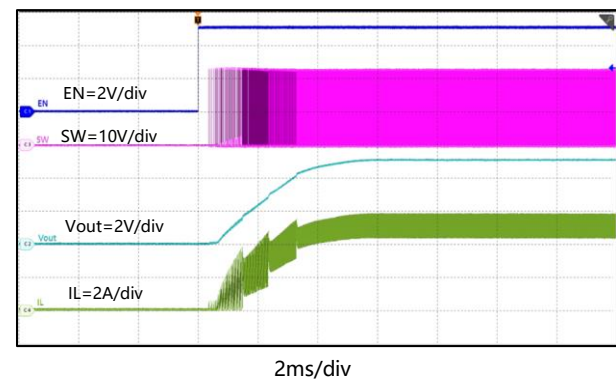
Figure 39. Start-Up with EN, I_{OUT}=5\text{A}
