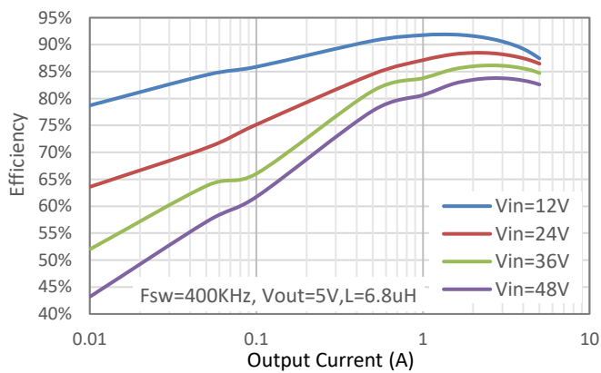
Figure 3. Power Efficiency, V_{out}=5V
