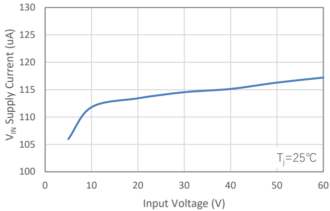
Figure 13. VIN Supply Current vs Input Voltage
