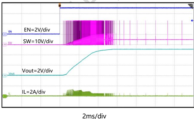
Figure 38. Start-Up with EN, I_{OUT}=0\text{A}
