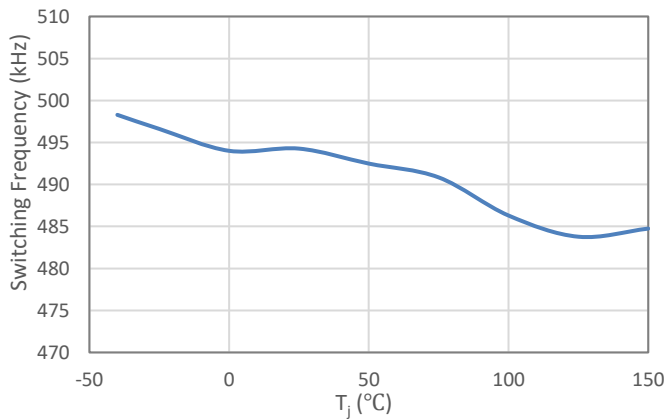
Figure 9. Switching Frequency vs Junction Temperature
