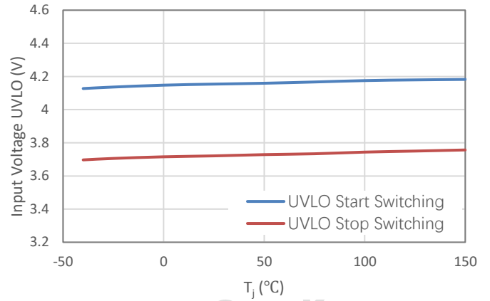
Figure 20. Input Voltage UVLO vs Junction Temperature
