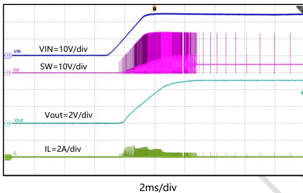
Figure 42. Start-Up with VIN rising, I_{OUT}=0A
