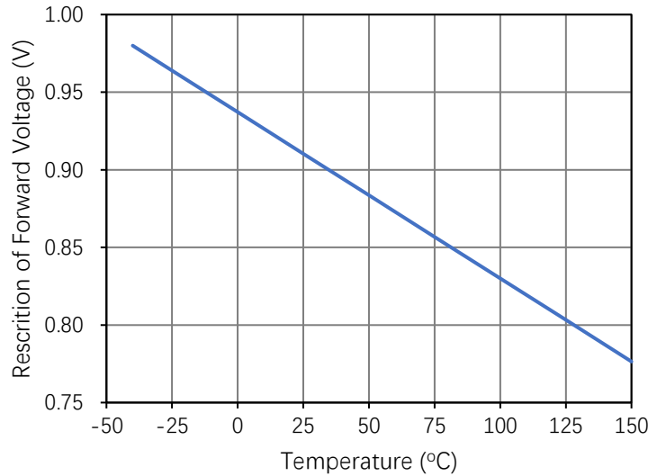
Figure 33. Restriction of Forward Voltage vs. Temperature
