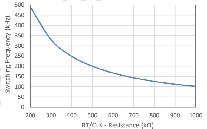
Figure 10. Switching Frequency vs RT/CLK Resistance Low Frequency Range
