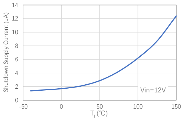
Figure 21. Shutdown Supply Current vs Junction Temperature
