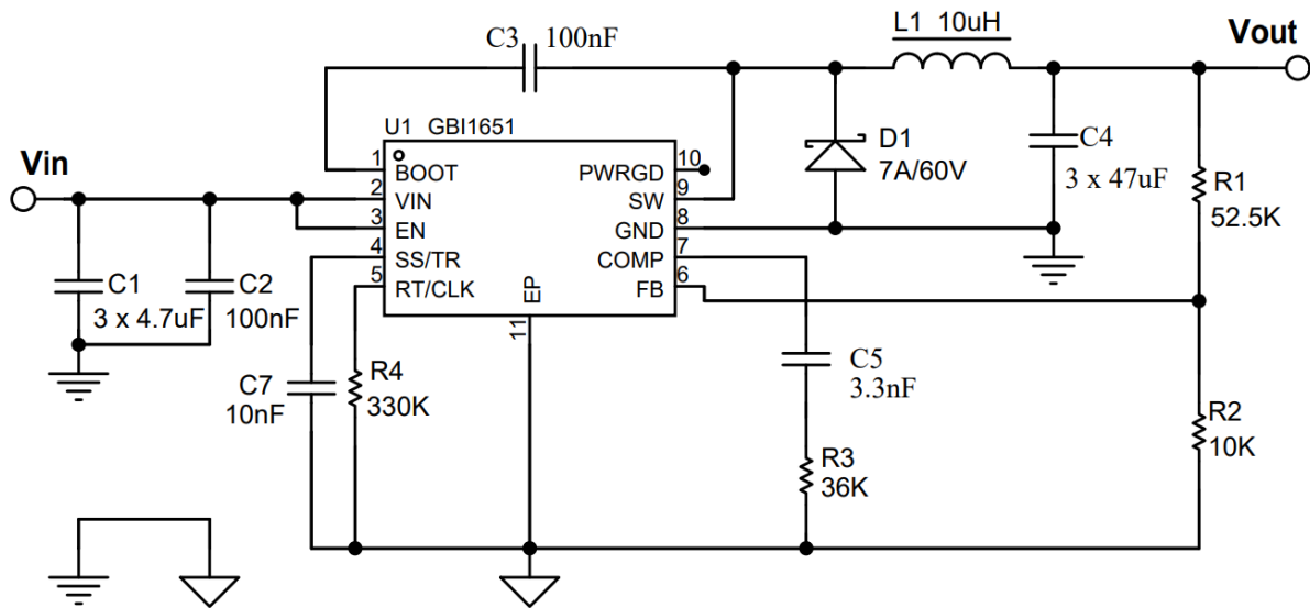
Figure 32. 24V Input, 5V/5A Output
