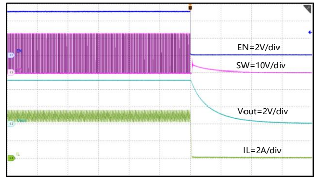
Figure 41. Shut-down with EN, I_{OUT}=5A
