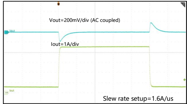
Figure 27. Transient Response 0.5A-4.5A
