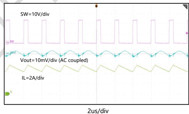
Figure 17. Output Voltage Ripple, I_{OUT}=5\text{A}
