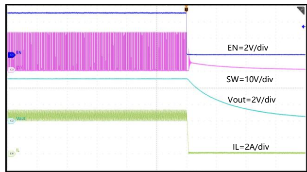
Figure 21. Shut-down with EN, I_{OUT}=5A
