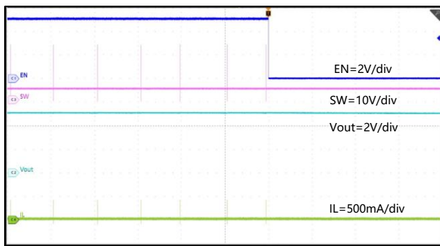
Figure 20. Shut-down with EN, I_{OUT}=0A
