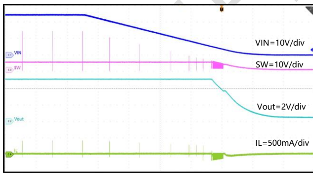
Figure 24. Shut-Down with VIN falling, I_{OUT}=0A
