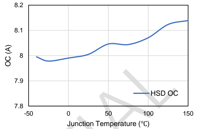
Figure 8. Over Current
