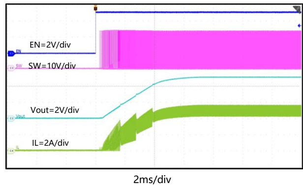
Figure 19. Start-Up with EN, I_{OUT}=5\text{A}
