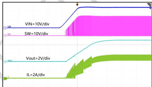
Figure 23. Start-Up with VIN Rising, I_{OUT}=5A
