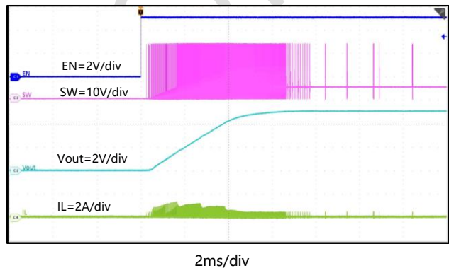
Figure 18. Start-Up with EN, I_{OUT}=0\text{A}
