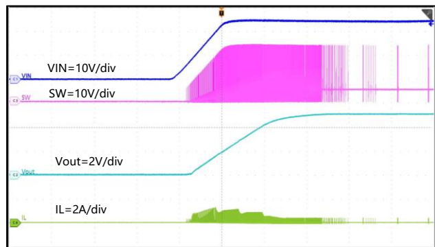
Figure 22. Start-Up with VIN rising, I_{OUT}=0A
