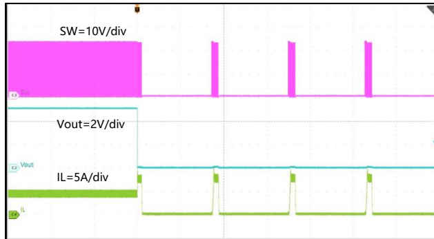
Figure 28. Normal Operation to Hard-short I OUT =5A
