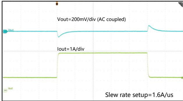
Figure 26. Transient Response 1.25A-3.75A
