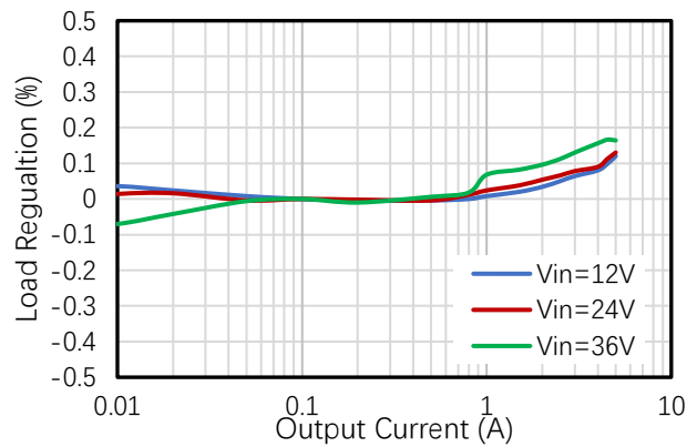
Figure 15. Load Regulation
