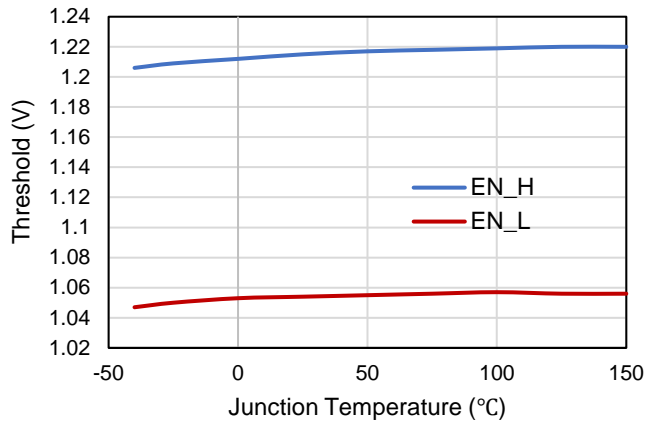
Figure 7. Enable Threshold
