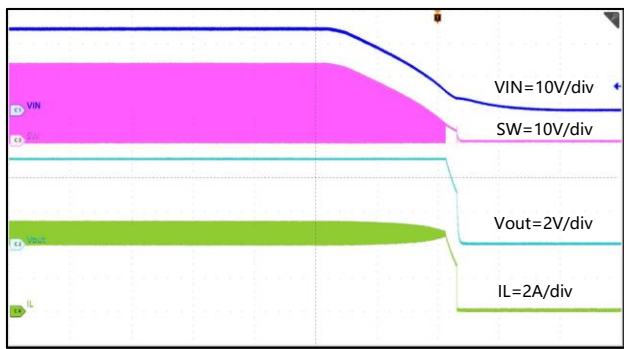
Figure 25. Shut-Down with VIN falling, I_{OUT}=5A
