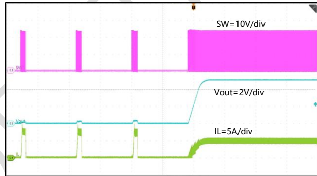
Figure 29. Hard-short Recover I OUT =5A
