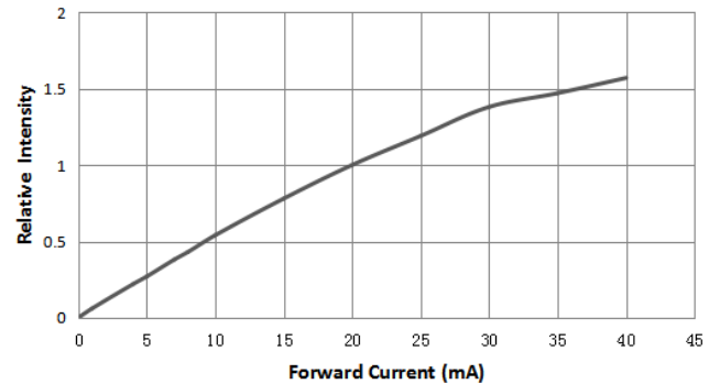
Relative Intensity VS. Forward Current ( T_a=25^\circ\text{C} )
