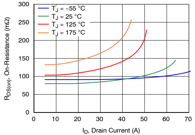
Figure 8. Typical Drain-Source On-Resistance V_{GS} = 0 V
