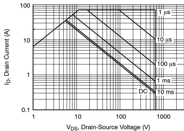
Figure 12. Safe Operation Area at T_C = 25 °C, Parameter t_p
