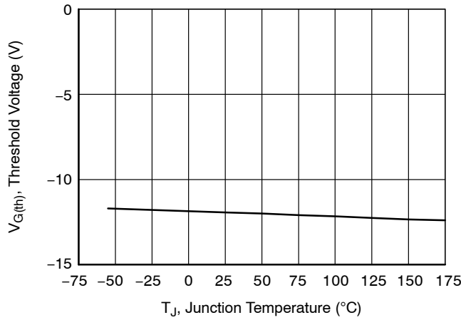
Figure 9. Threshold Voltage vs. T_J at V_{DS} = 5 V and I_D = 20 mA
