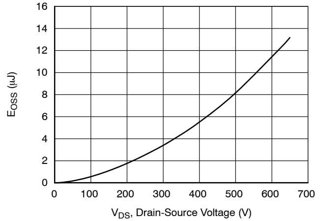
Figure 10. Typical Stored Energy in C_{OSS} at V_{GS} = -20 V
