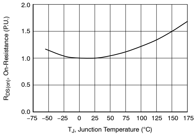
Figure 7. Normalized On-Resistance Vs. Temperature at V_{GS} = 0 V and I_D = 10 A
