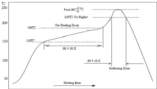
回流焊 (IR Reflow Soldering)
