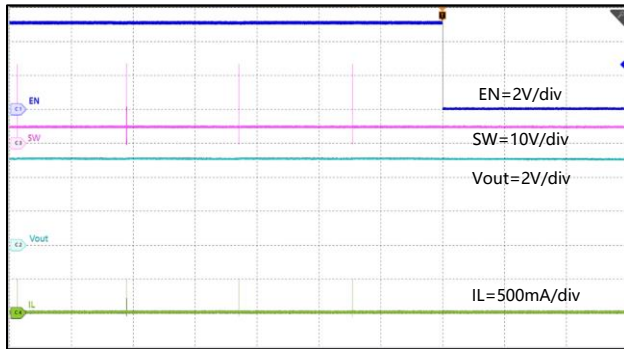
Figure 38. Shut-down with EN, I_{OUT}=0A
