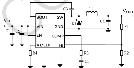
Simplified Schematic
