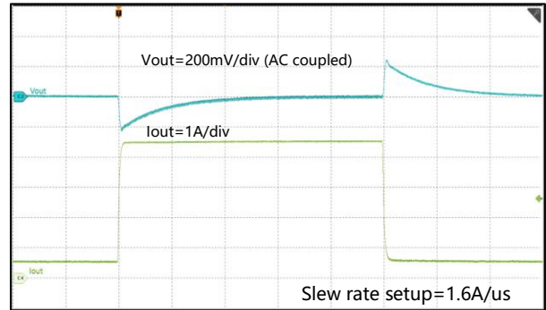
Figure 45. Transient Response 0.5A-4.5A
