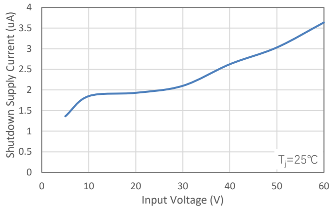
Figure 21. Shutdown Supply Current vs Input Voltage
