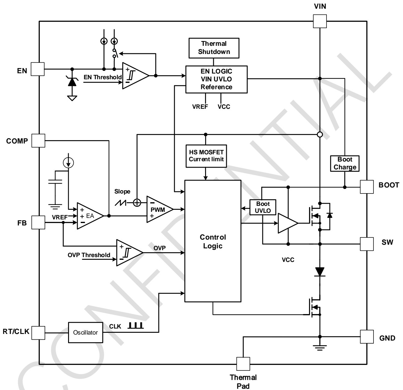
Figure 25 Block Diagram of GBI1650
