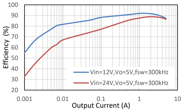
Figure 32. Power Efficiency
