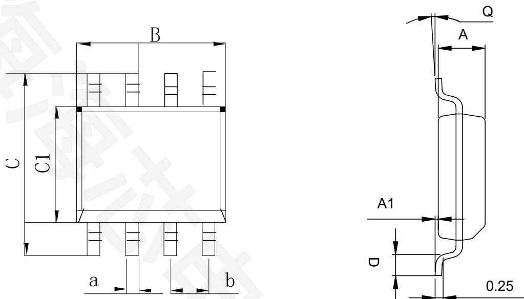
Dimensions In Millimeters(SOP8)
