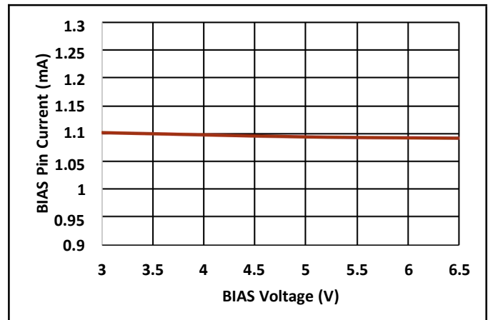
Fig. 6 BIAS Pin Current vs BIAS Voltage
