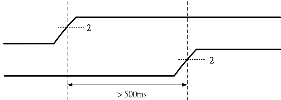
Figure 4 PERST_N sequence
