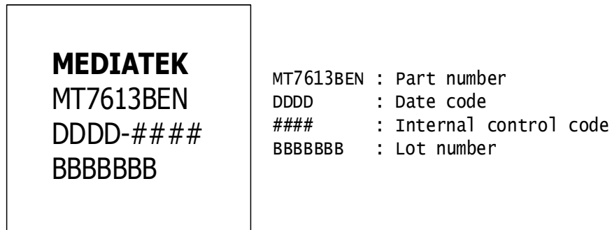
Figure 8 MT7613BEN Top Marking
