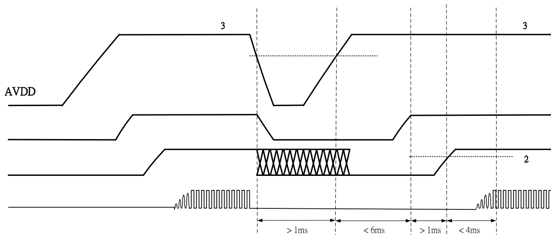
Figure 3 Cold reset sequence
