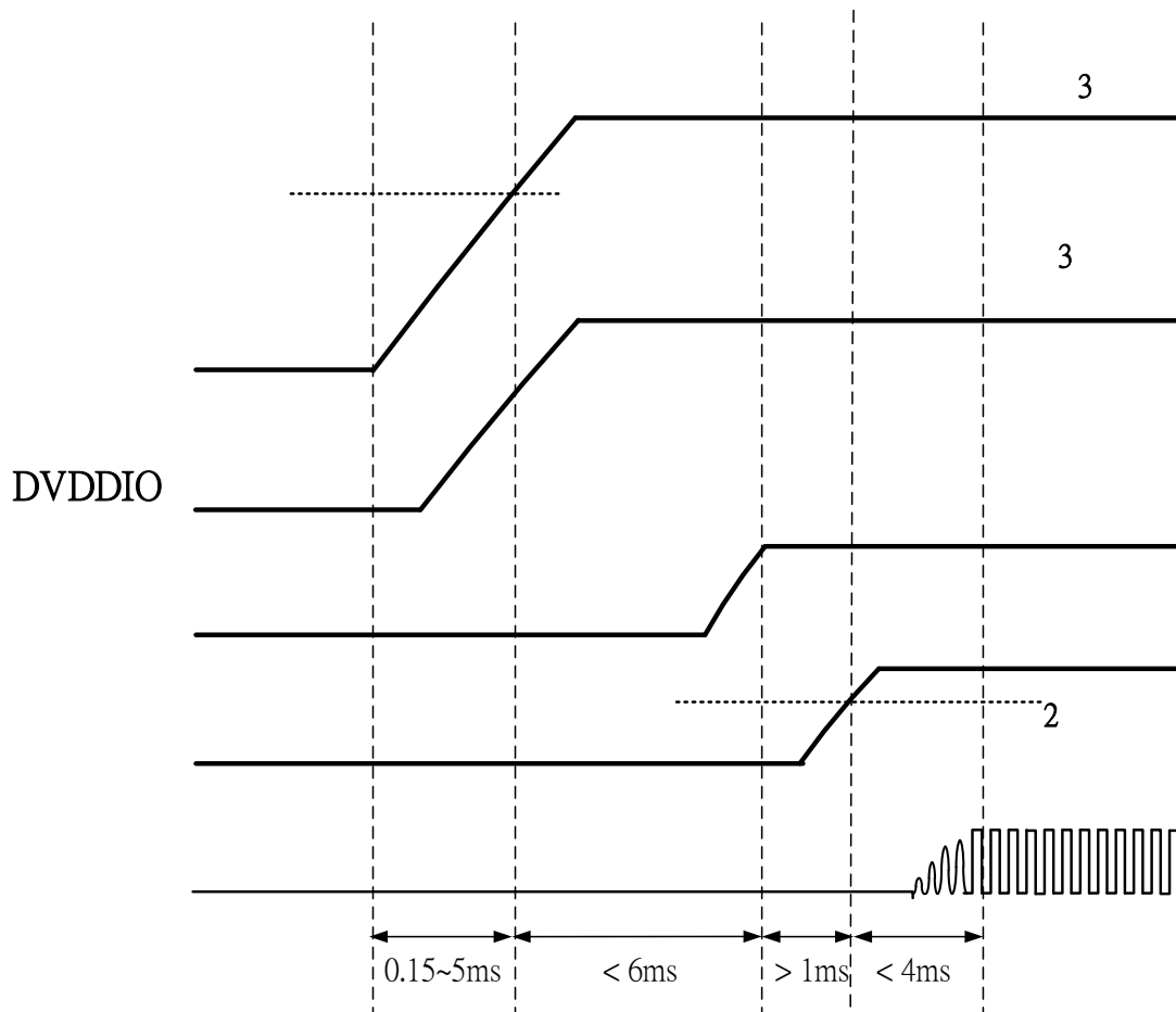
Figure 2 Chip power on sequence
