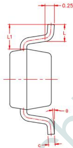
RIGHT-VIEW:
