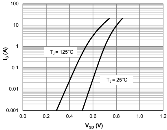
Figure 7: Body-Diode Characteristics
