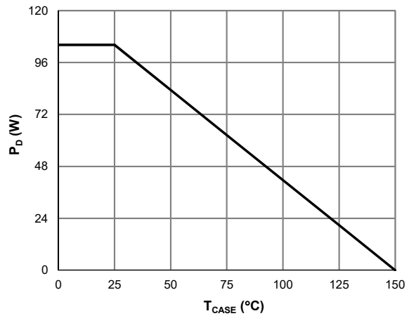
Figure 10: Power De-rating
