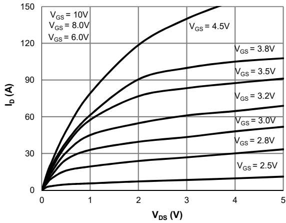
Figure 1: Saturation Characteristics
