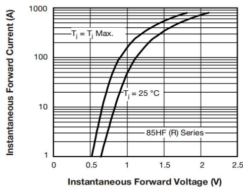
Fig. 12 - Forward Voltage Drop Characteristics (for 1400 V, 1600 V)
