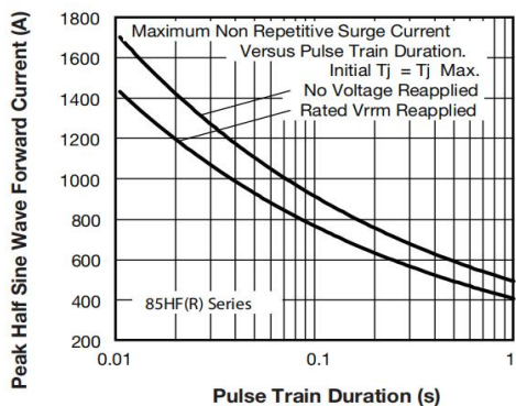
Fig. 10 - Maximum Non-Repetitive Surge Current
