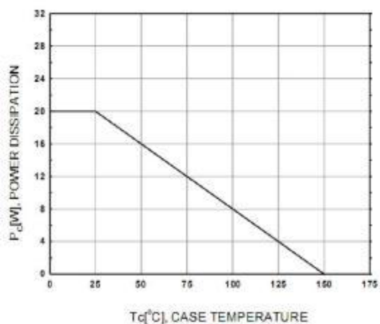
Figure 5. Power Derating
