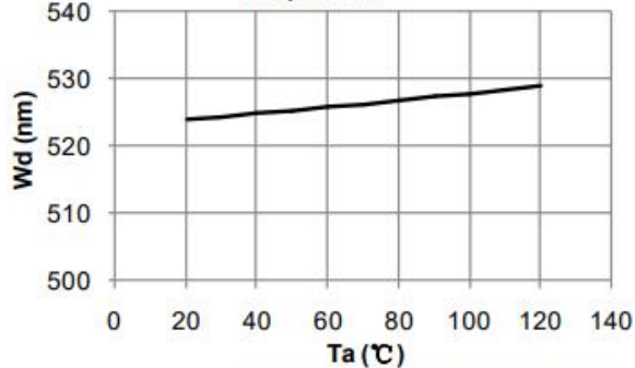
Fig.5-Dominant Wavelength (@120mA) vs. Ambient Temperature
