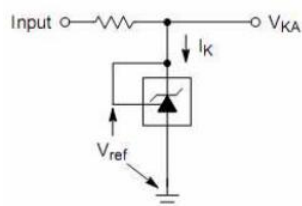
Test Circuit for V_{KA} = V_{ref}
