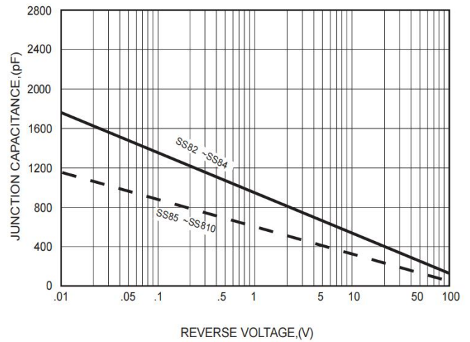
FIG.4-TYPICAL JUNCTION CAPACITANCE
