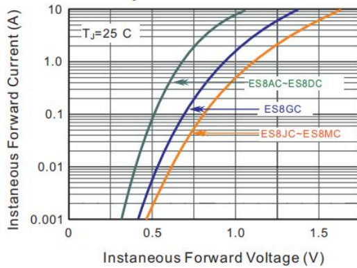
FIG.3-TYPICAL FORWARD CHARACTERISTICS
