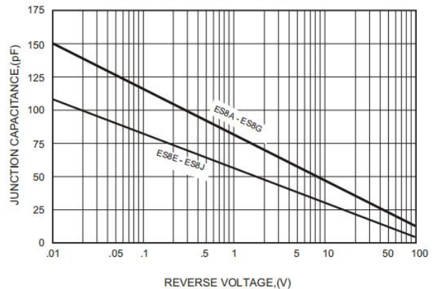
FIG.6-TYPICAL JUNCTION CAPACITANCE
