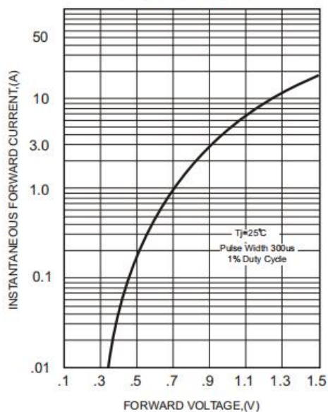
FIG.2-TYPICAL FORWARD CHARACTERISTICS
