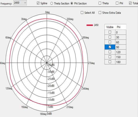
\phi = 90^\circ Plane YZ at 2450 MHz, Gain -1.02dBi
