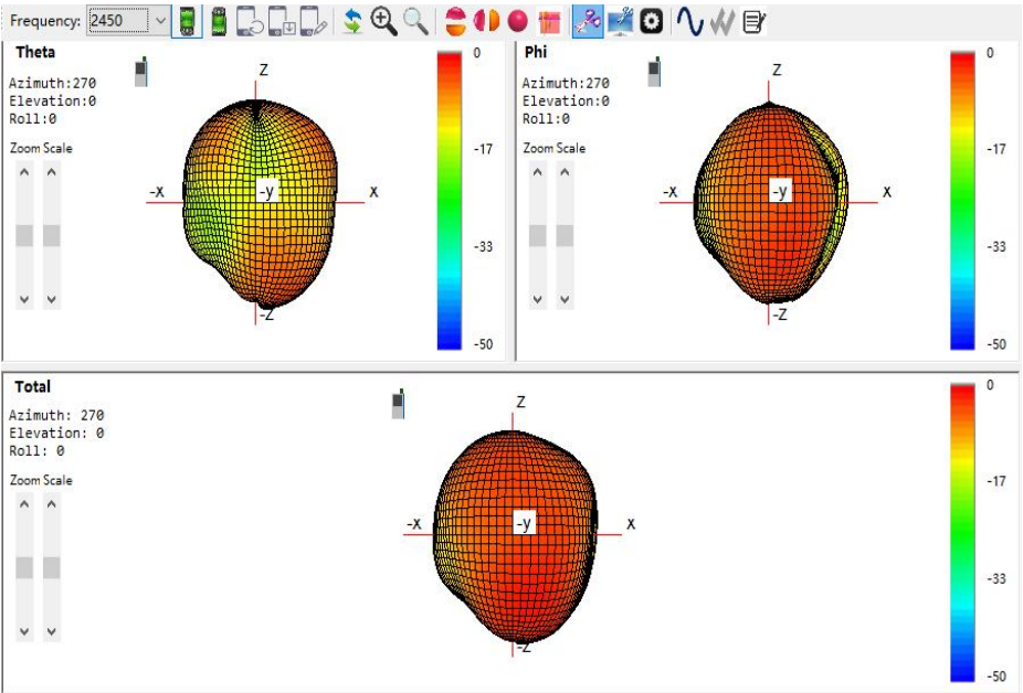
\phi = 0^\circ Plane XZ at 2450 MHz, Gain -1.02 dBi
