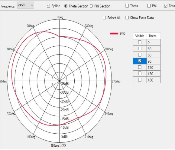
\theta = 90^\circ Plane XY at 2450 MHz, Gain -1.02 dBi
