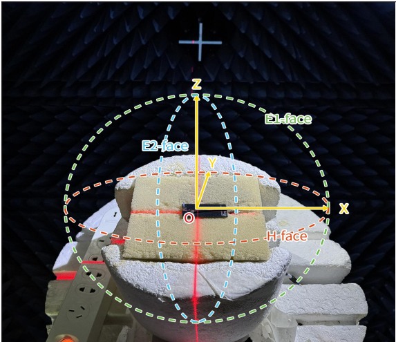
PCB board size: 45 mm x 20 mm x 1.2 mm
