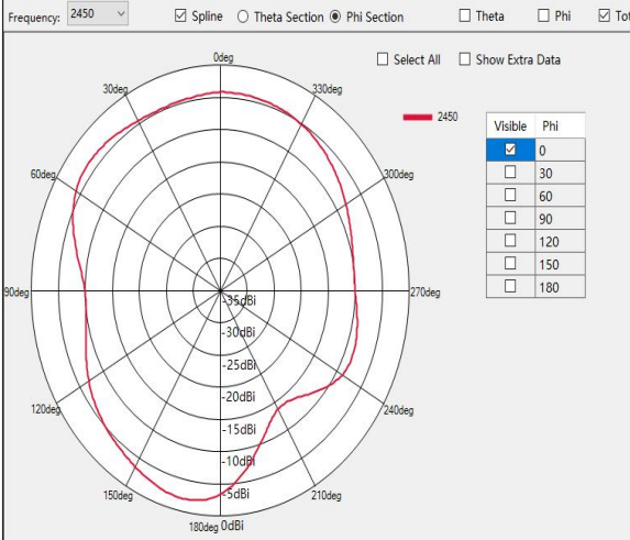
\phi = 0^\circ Plane XZ at 2450 MHz, Gain -1.02 dBi
