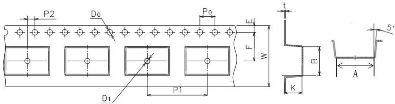
料带尺寸Material belt size
