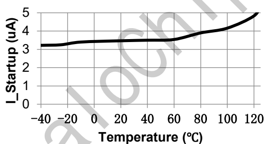
I_Startup vs. Temperature
