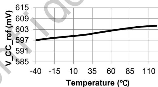
V_CC_ref vs Temperature
