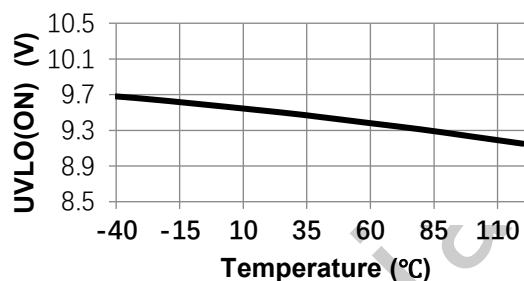
UVLO(ON) vs Temperature
