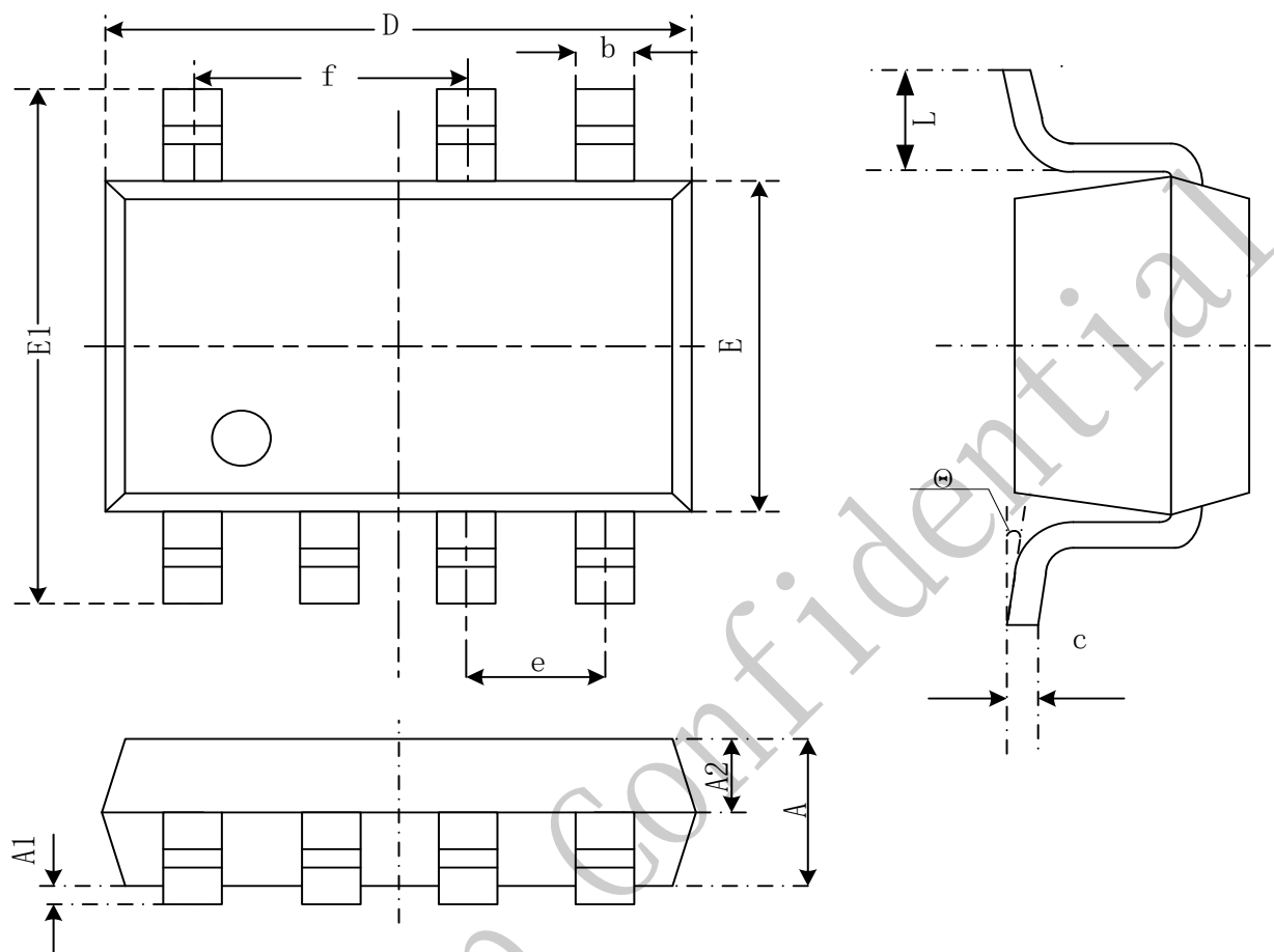
SOP7 PACKAGE OUTLINE DIMENSIONS
