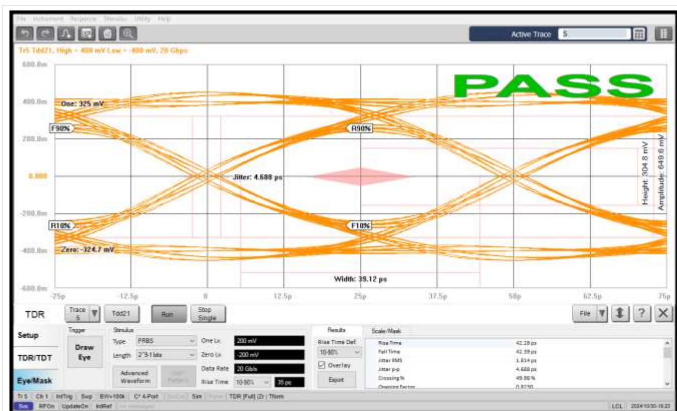
20 Gbps HDMI 2.1 Eye Diagram
