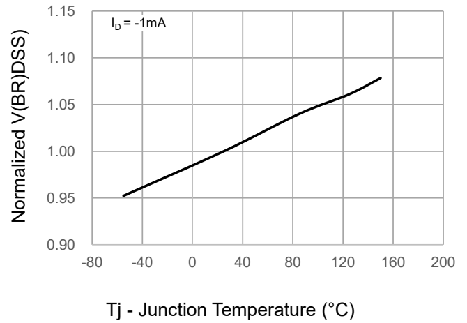
Fig2. Normalized Threshold Voltage Vs. Temperature
