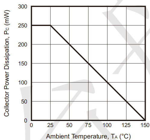
Fig.7 - P_C — T_A
