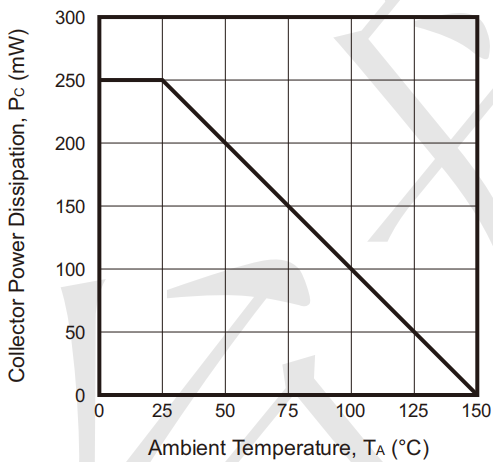
Fig.7 - P_C — T_A
