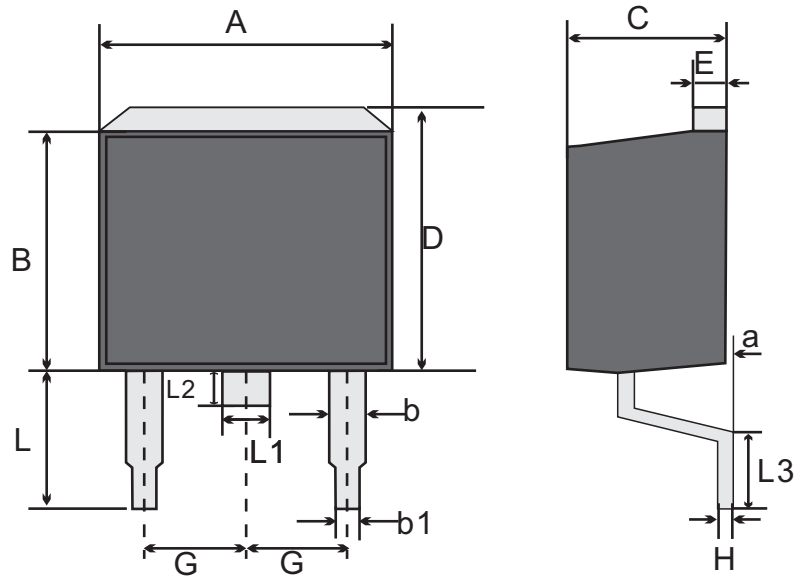
TO-263(D 2 PAK) mechanical data
