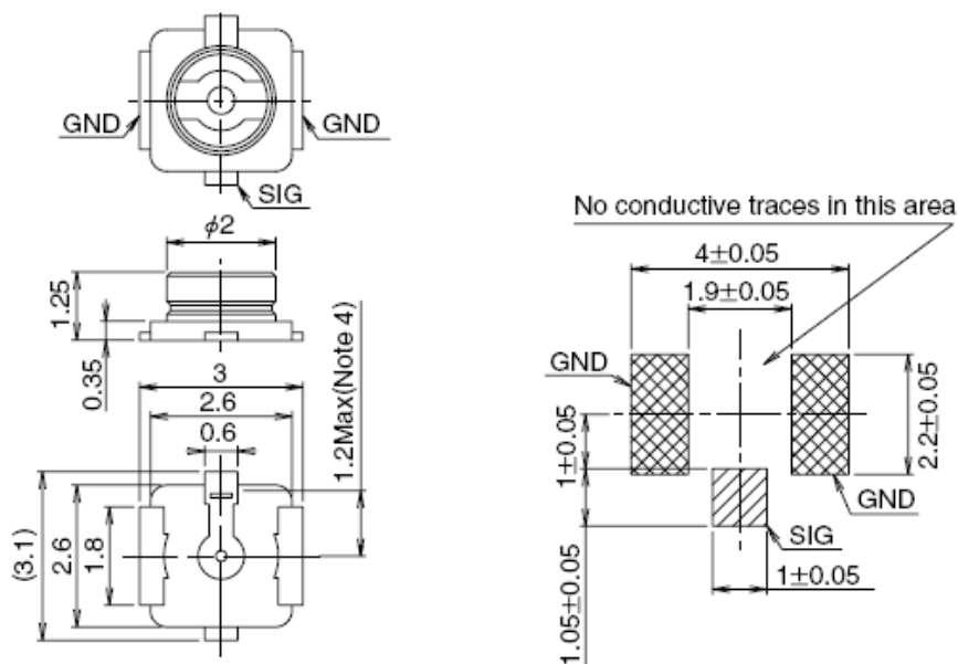
Figure 33: Dimensions of the Receptacle (Unit: mm)
