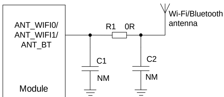
Figure 28: Reference Design for Wi-Fi/Bluetooth Antenna Interface
