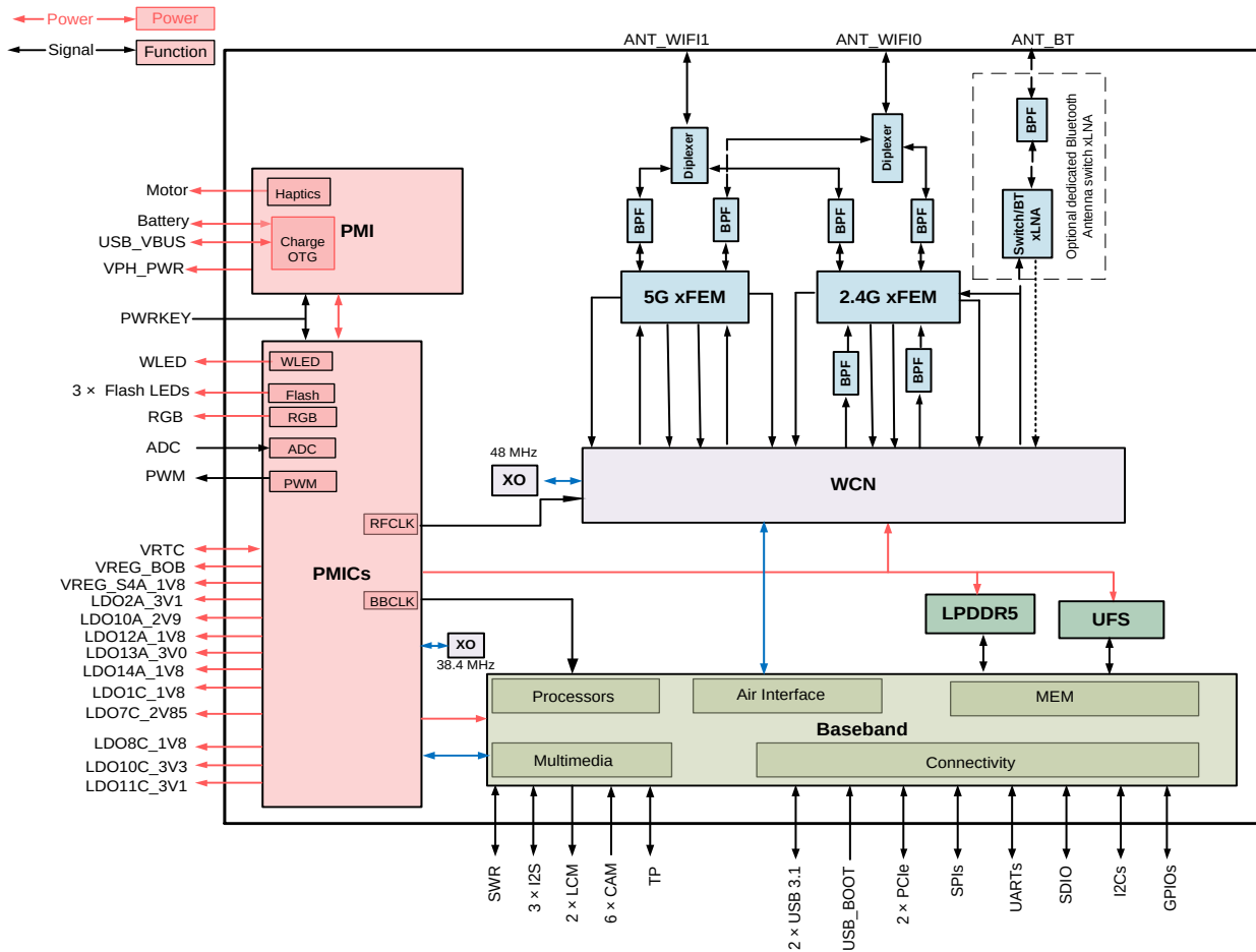
Figure 1: Functional Diagram
