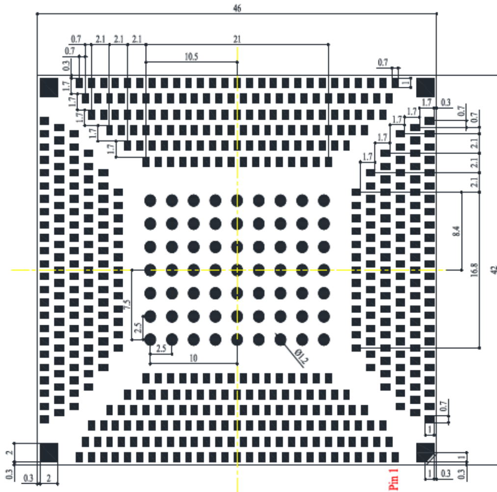
Figure 37: Module Bottom Dimensions (Bottom View)
