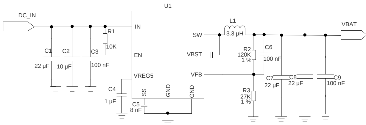
Figure 4: Reference Circuit of Power Supply
