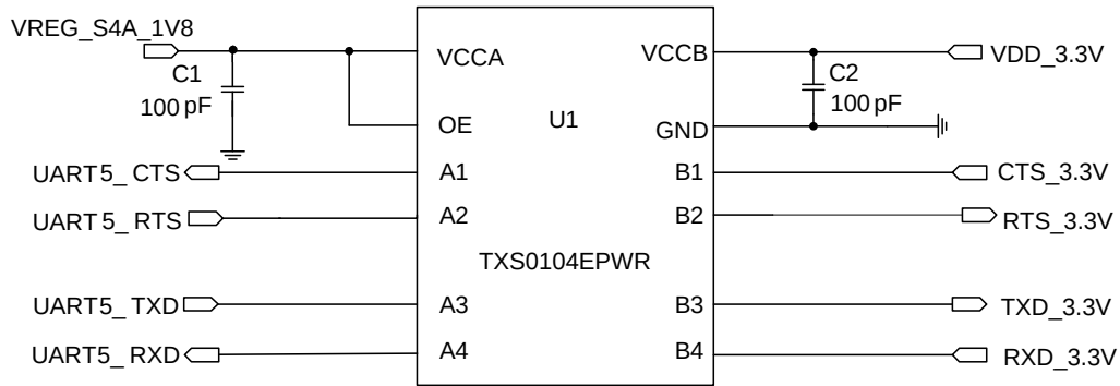
Figure 16: Reference Circuit with Voltage-level Translator Chip (for UART 5)
