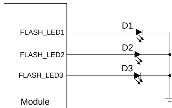
Figure 26: Reference Design for Flashlight Interfaces
