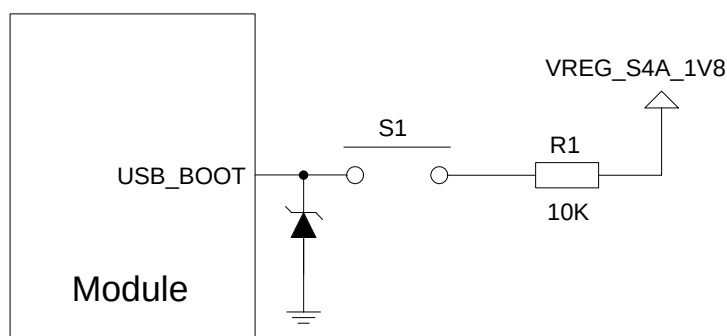
Figure 27: Reference Design for USB_BOOT
