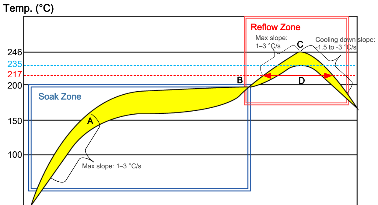
Figure 40: Recommended Reflow Soldering Thermal Profile
