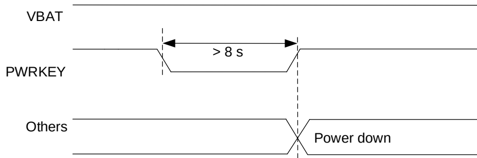
Figure 11: Forced Power-down Timing
