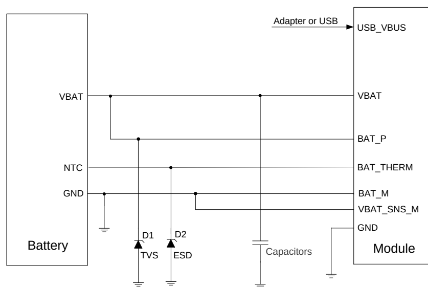
Figure 3: Reference Design for Battery Charging Circuit
