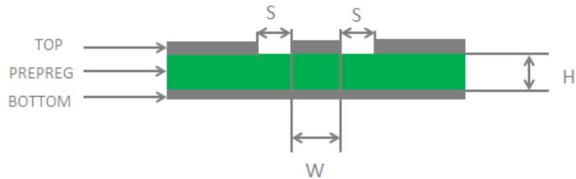
Figure 30: Coplanar Waveguide Design on a 2-layer PCB
