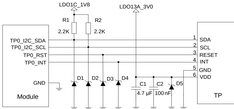
Figure 23: Reference Design for TP0 Interface
