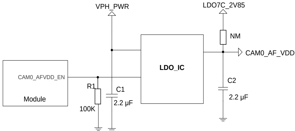
Figure 25: Reference Design of Camera Power Supply
