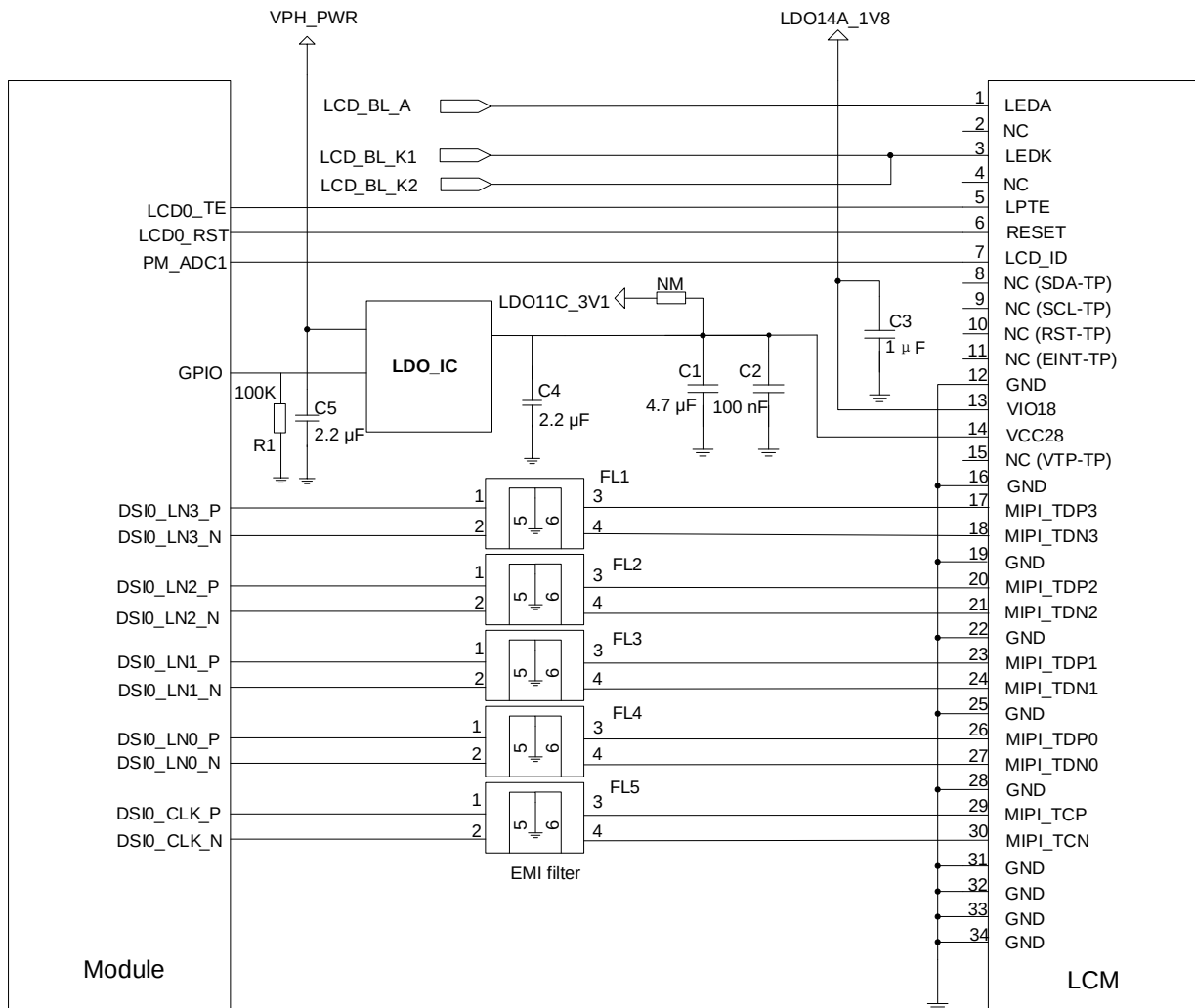
Figure 22: Reference Design for LCM0 Interface
