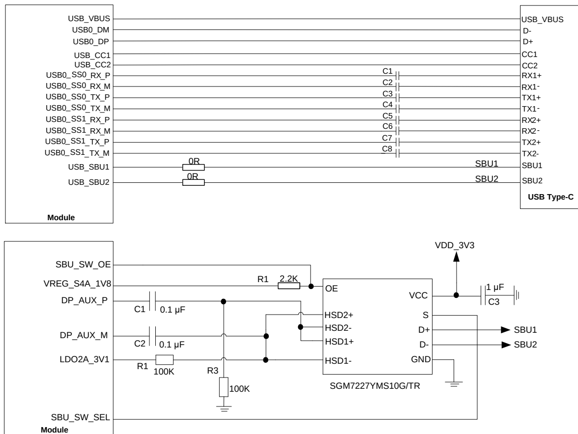
Figure 15: Reference Design for DisplayPort Mode
