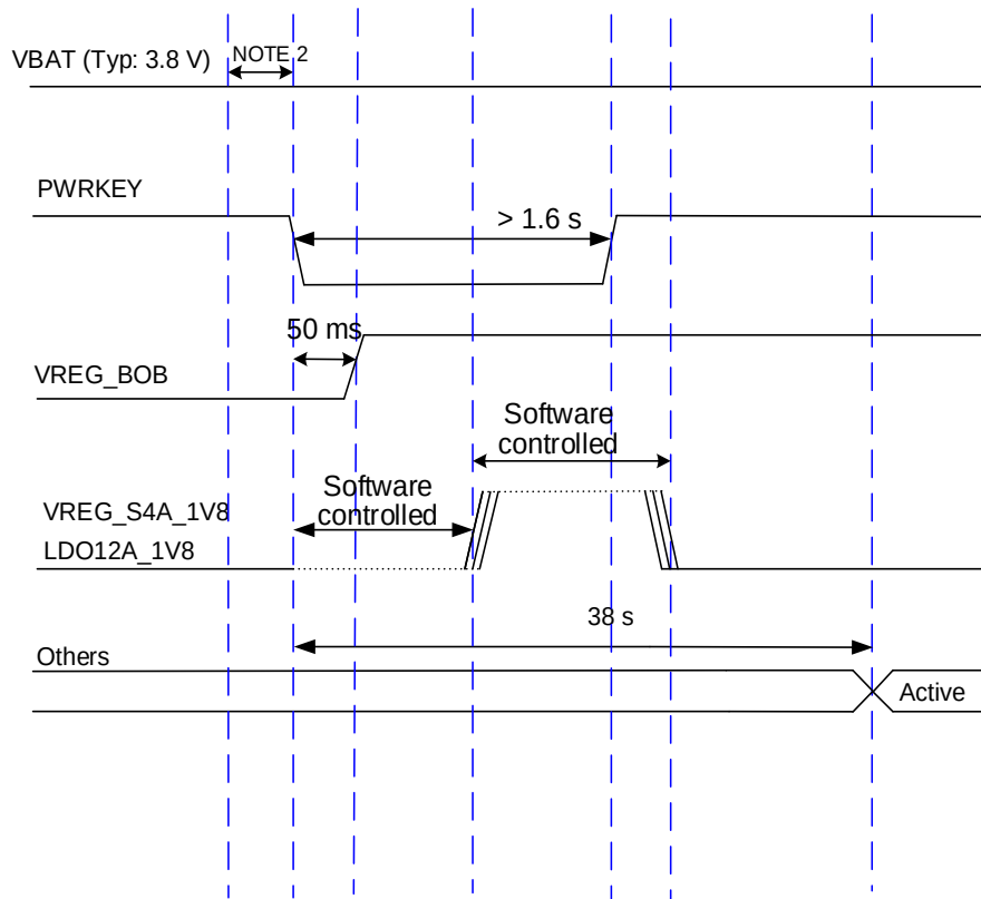
Figure 10: Power-up Timing
