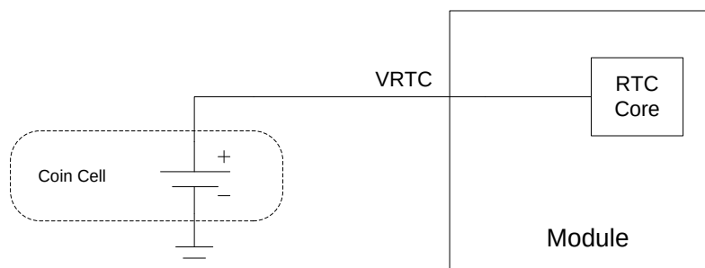
Figure 12: RTC Powered by a Coin Cell
