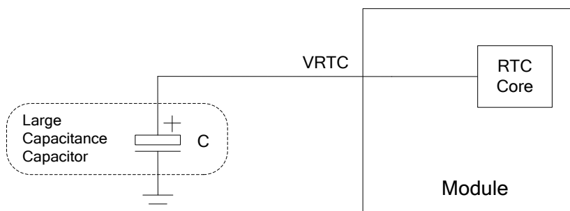
Figure 13: RTC Powered by Capacitor
