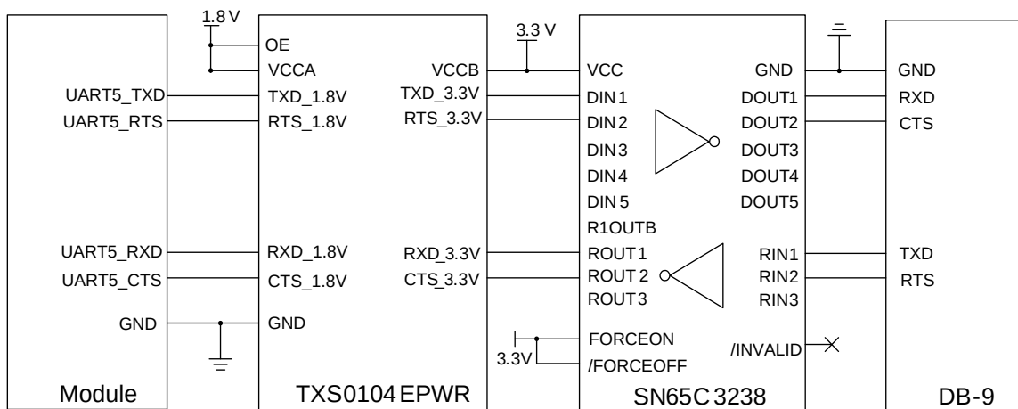
Figure 17: RS-232 Level Matching Circuit (for UART 5)
