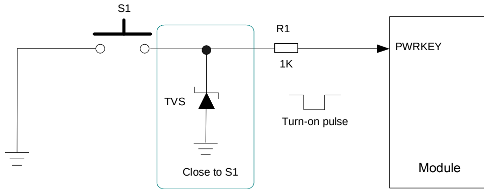
Figure 8: Turn On the Module Using a Button
