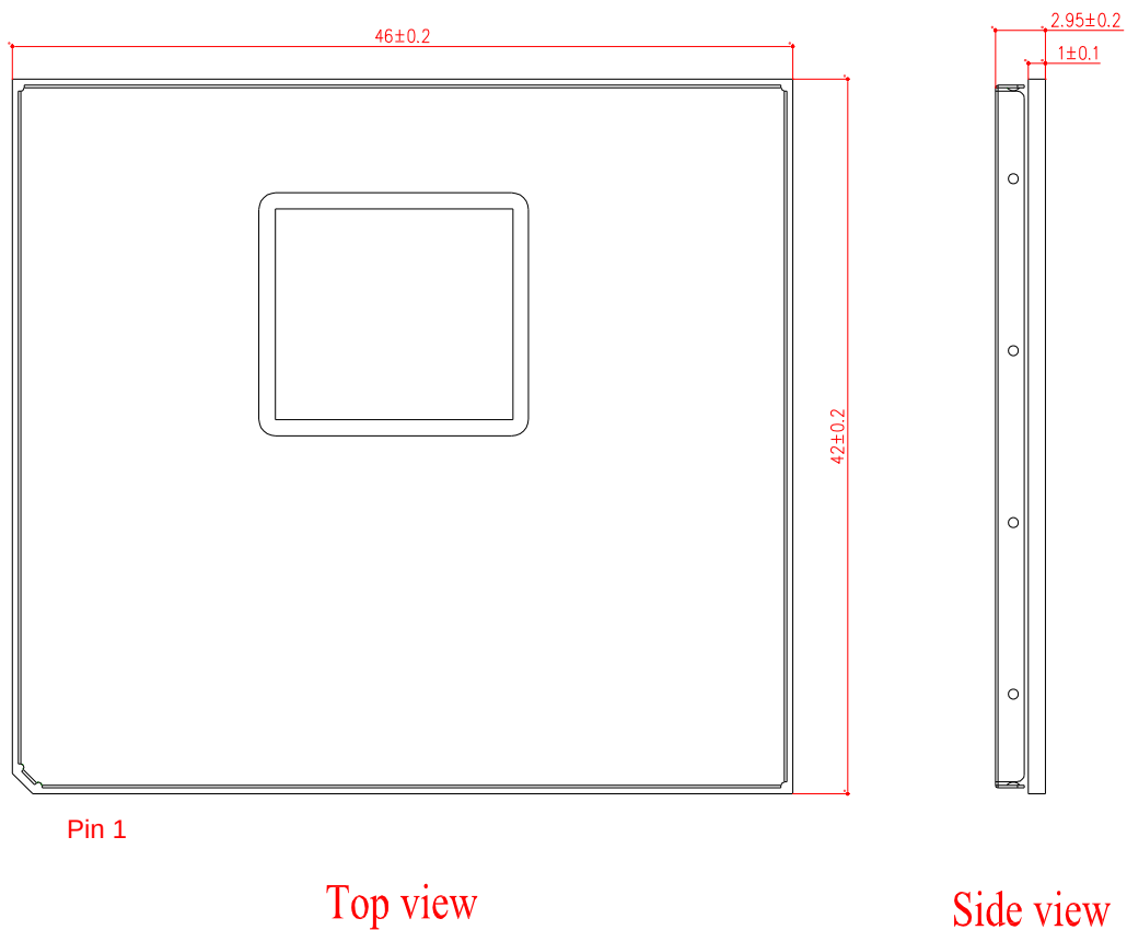
Figure 36: Module Top and Side Dimensions
