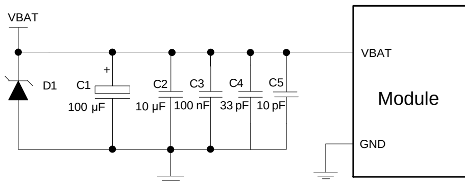
Figure 6: Structure of Power Supply
