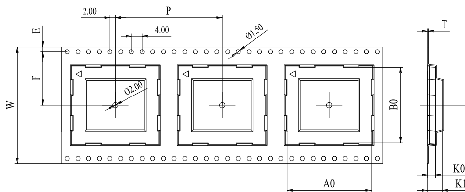
Figure 41: Carrier Tape Dimension Drawing
