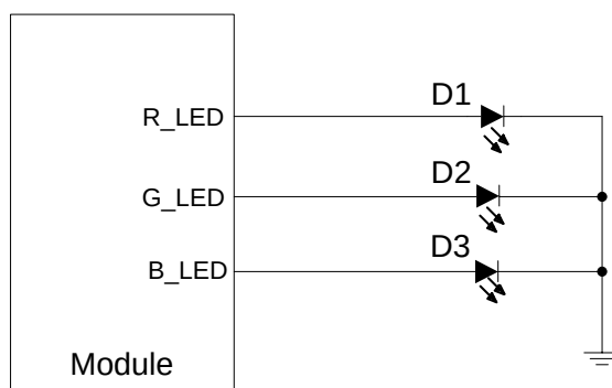
Figure 21: Reference Design for RGB Interfaces
