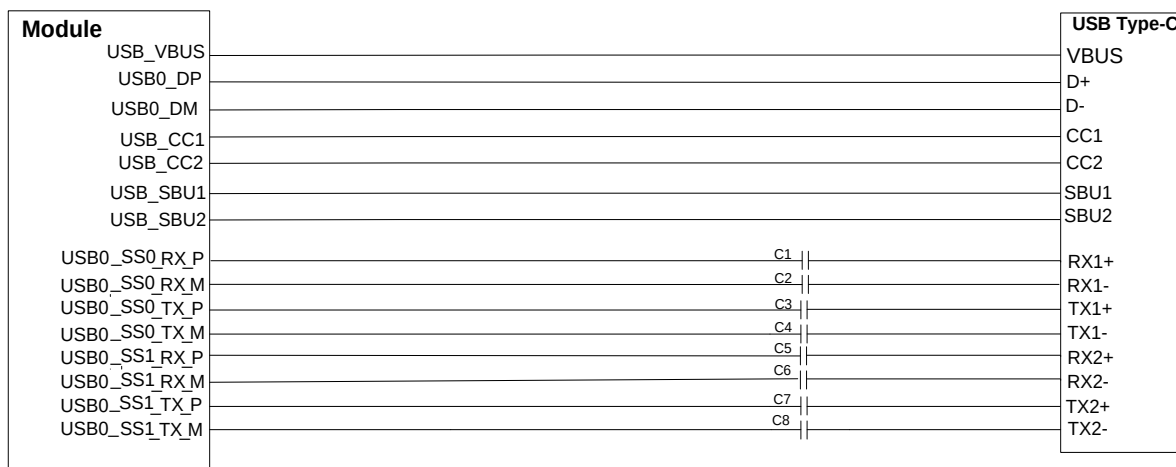
Figure 14: USB Type-C Interface Reference Design
