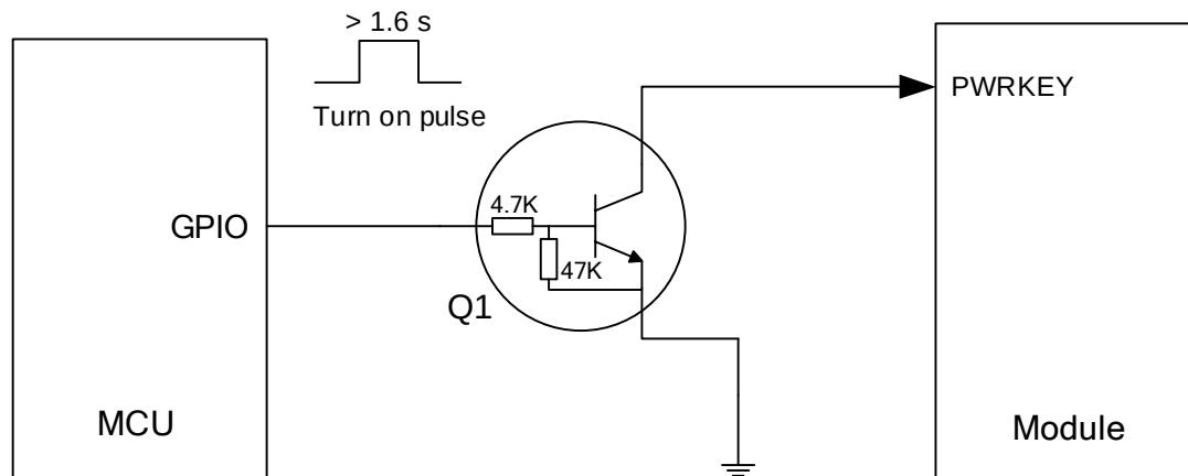
Figure 7: Turn On the Module Using Driving Circuit
