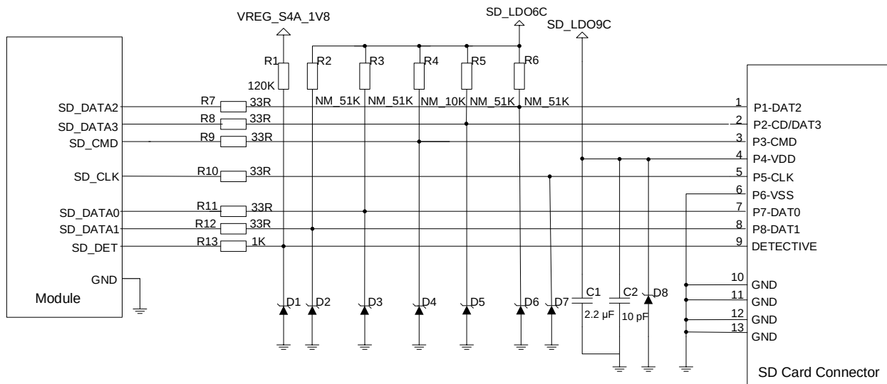
Figure 18: Reference Circuit for SD Card Interface
