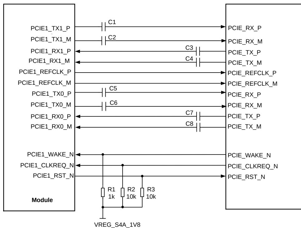
Figure 19: Reference Design of PCIe1 Interface
