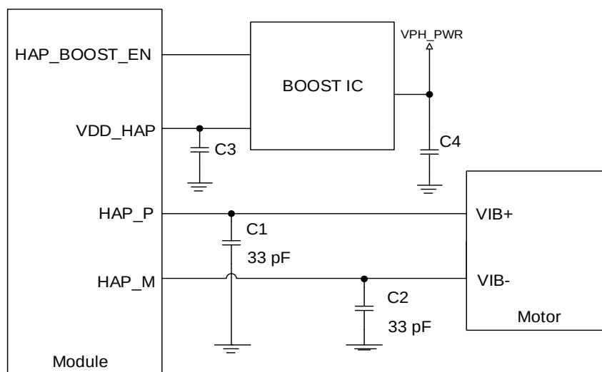
Figure 20: Reference Design for Vibrator Connection
