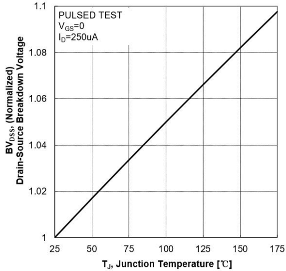
Figure 5 BV vs Junction Temperature
