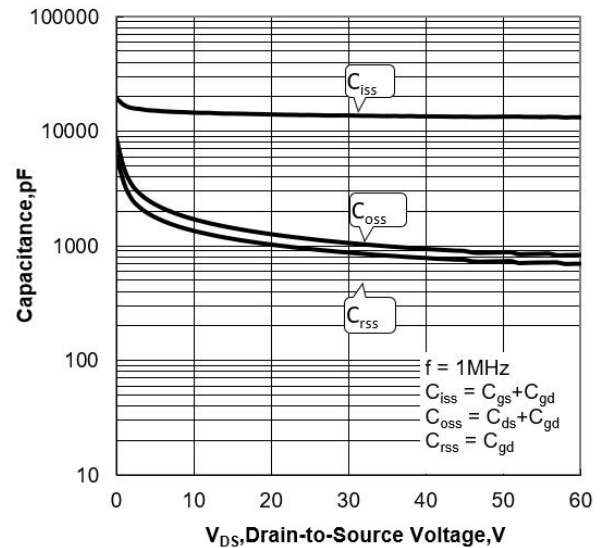
Figure 8 Capacitance Characteristics
