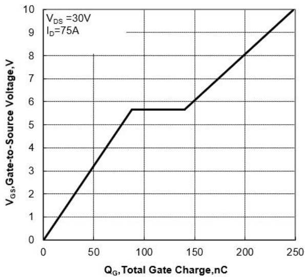
Figure 7 Gate-Charge Characteristics
