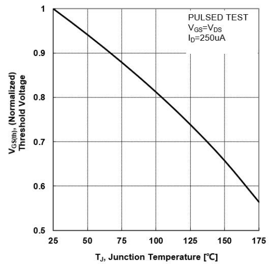
Figure 6 Vth vs Junction Temperature
