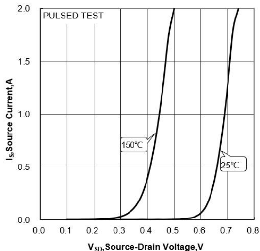
Figure 9 Body Diode Forward Voltage
