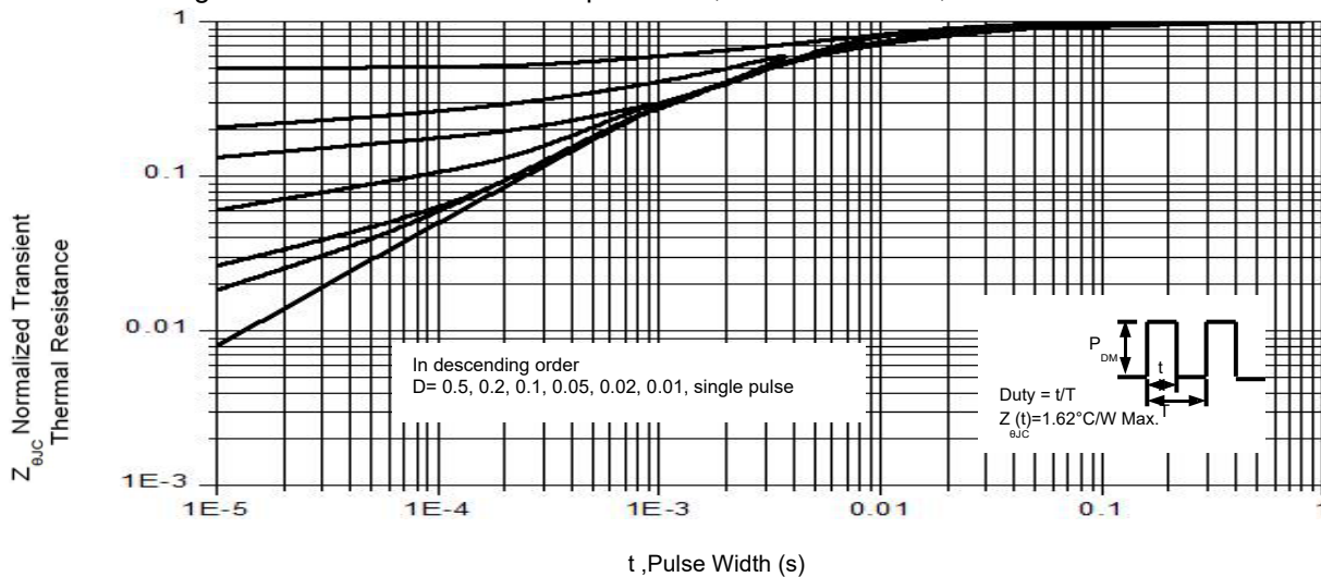
Figure 16. Transient Thermal Impedance, Junction to Case, TO-220/TO-252
