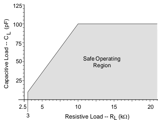
Figure 2. Maximum Loading
