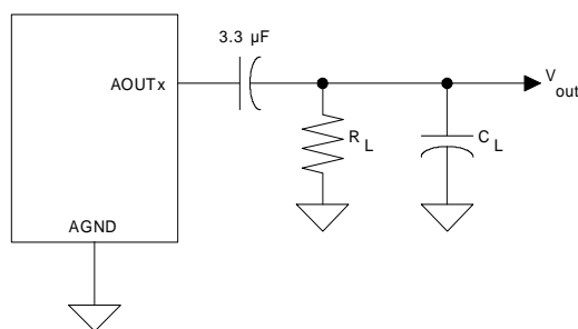
Figure 1. Output Test Load
