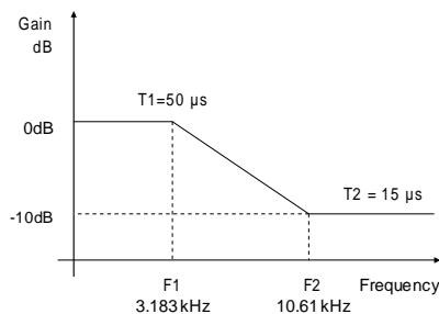
Figure 11. De-Emphasis Curve ( F_s = 44.1\text{kHz} )
