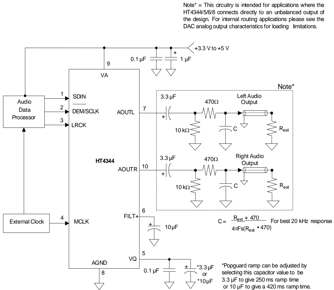
Figure 6. Recommended Connection Diagram
