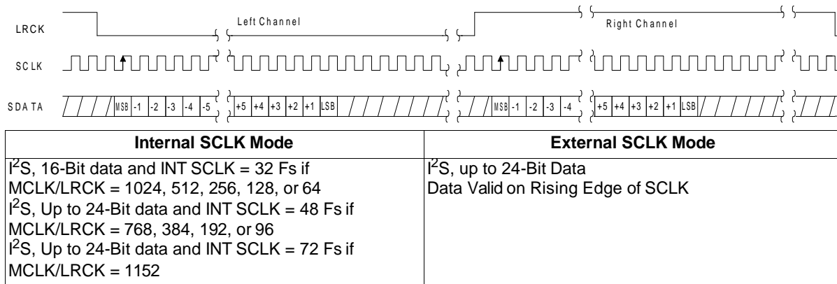
Figure 7. HT4344 Data Format ( I^2S )
