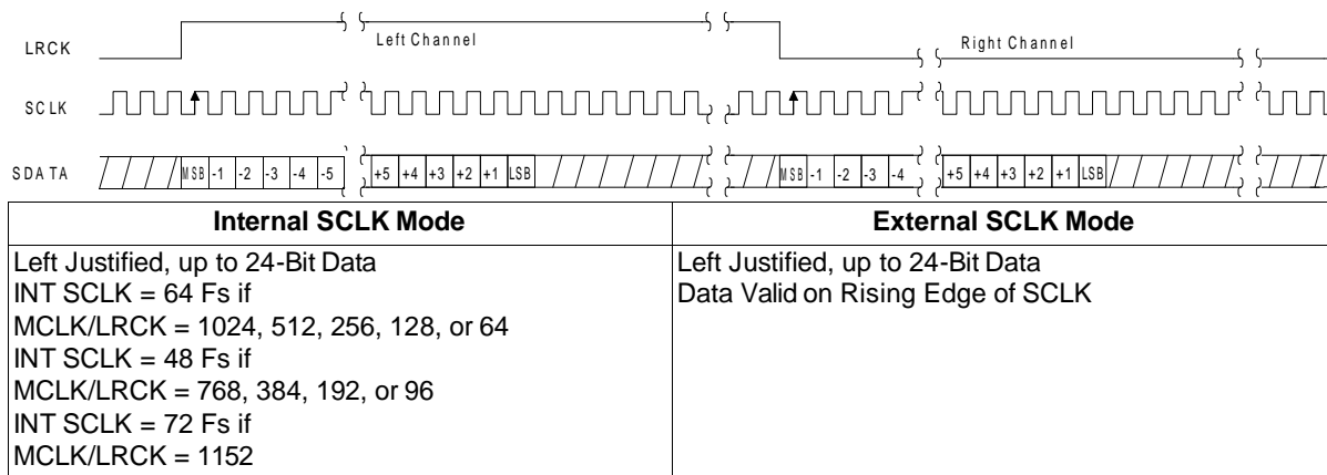
Figure 8. HT4345 Data Format (Left Justified)
