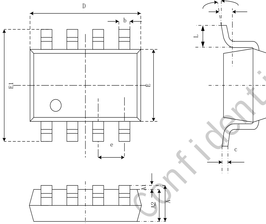
SOP8 PACKAGE OUTLINE DIMENSIONS
