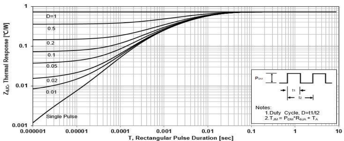
Figure 5. Transient Thermal Impedance
