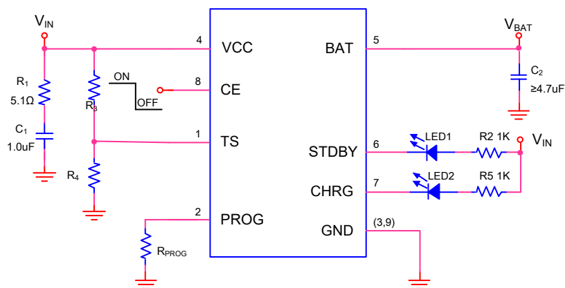
Figure 1. HE4056H Typical Application Circuit
