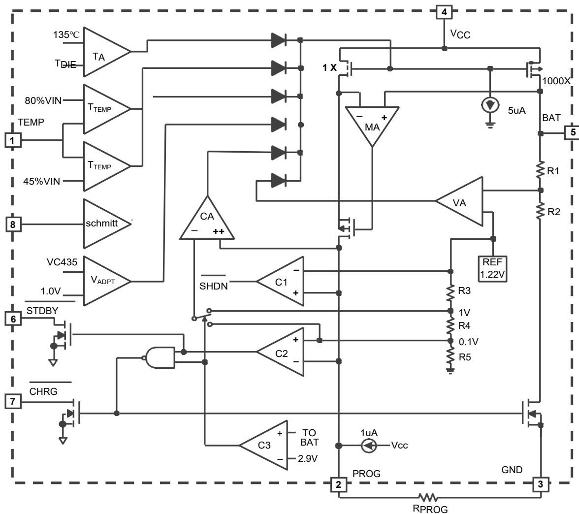
Figure 2. HE4056H Block Diagram
