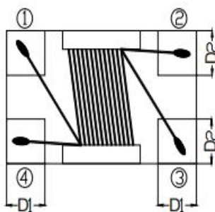
Recommended PC Board Pattern
