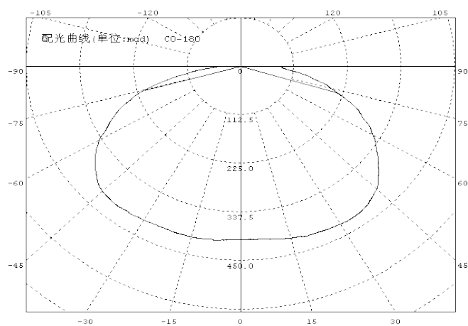
Directive Characteristics
