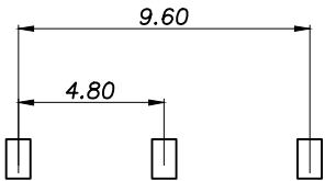
RECOMMENDED PCB LAYOUT GENERAL TOLERANCE ±0.05
