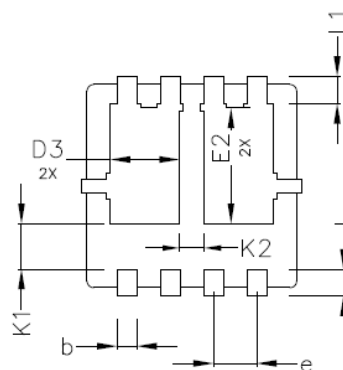
BOTTOM VIEW OPTION 2
